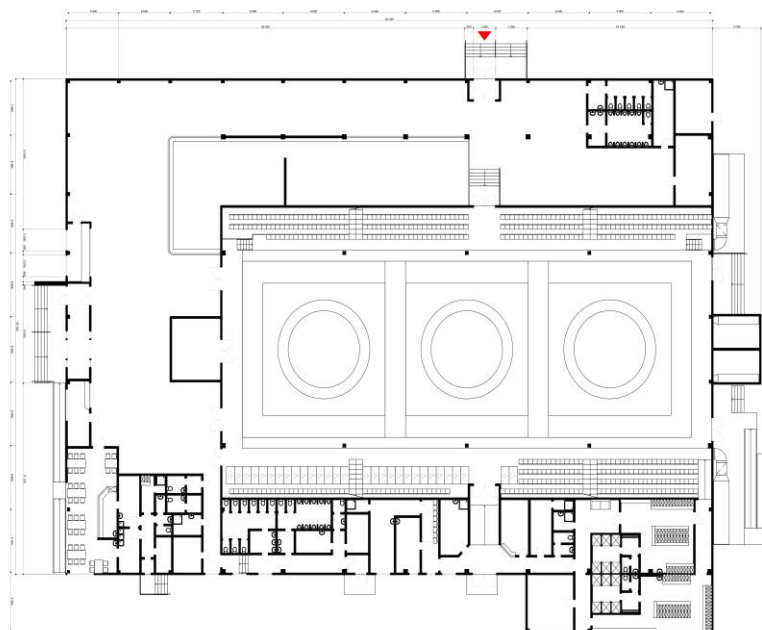
Fig. 1. The project of the multifunctional sports complex "Poddubny-Arena" in Yeysk.
